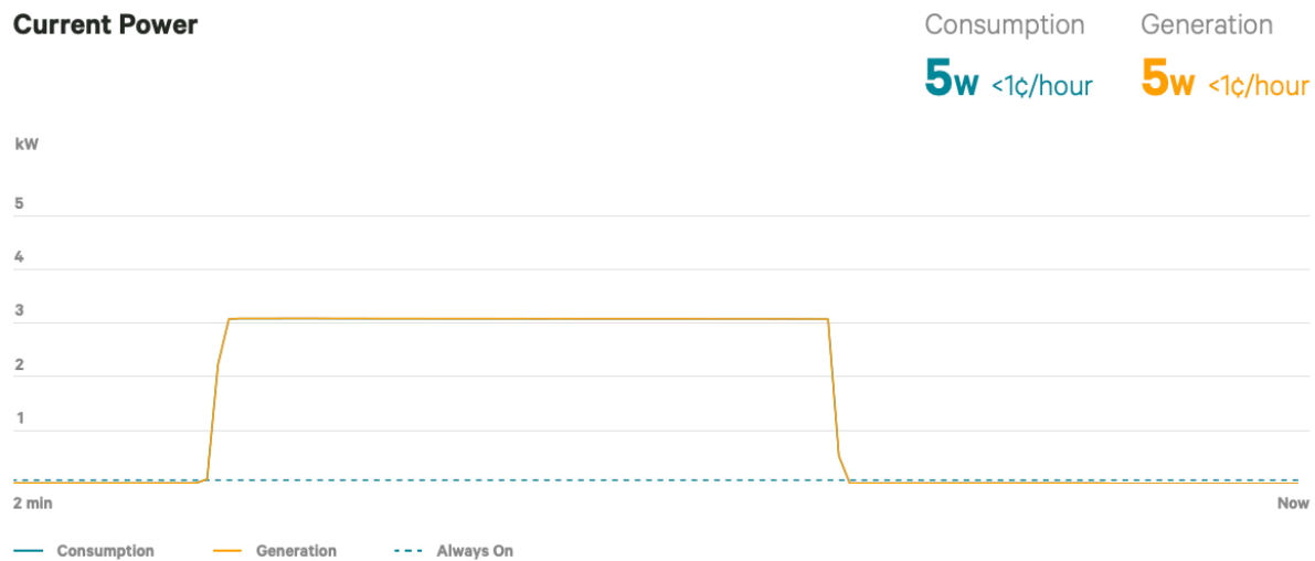
Figure 12. PWRView display, grid off. When the batteries have been fully charged by the solar, the solar is switched off (indicated by the very low kw level in the plot above) and the house load is serviced by the charged batteries, but when the batteries get low enough, the system switches to a charge state and are being charged by the solar. The solar will be charging batteries and the supplying the house, as well. The system goes back and forth between charging the batteries (and supplying part of the load) and running the house only from batteries. During fully charged state, where the battery voltage is between a preset high and low value, the SolarEdge power (from panels) is shut down.
